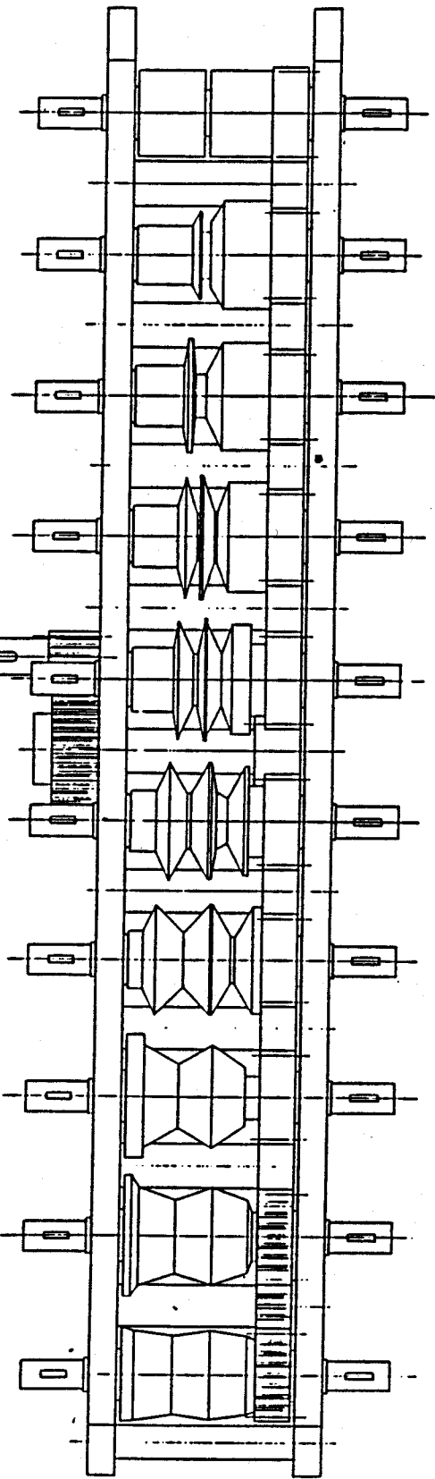
BOTTOM HEAD ASS'Y. FOR REINFORCED "S" CLEAT MACHINE
